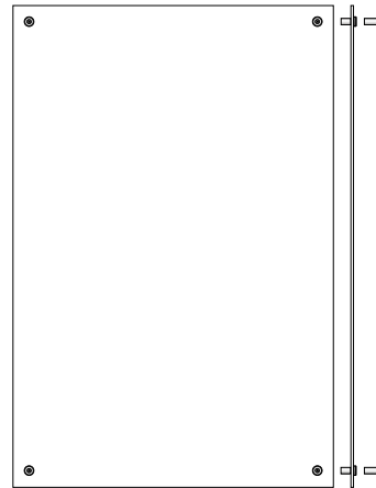
kit 115 V (kit A 30 / kit A 50) w 1000 x h 1500 x d 8mm w 39,37 x h 59,06 x d 0,31"
