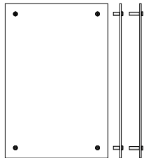
kit 106 V (kit B 30 / kit B 50) w 500 x h 750 x d 8mm w 19,69 x h 29,53 x d 0,31"
