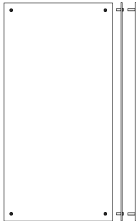
kit 113 V (kit B 30 / kit B 50) w 750 x h 1500 x d 8mm w 29,53 x h 59,06 x d 0,31"
