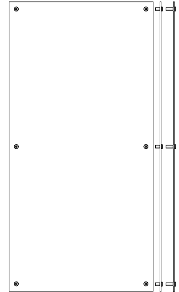
kit 120 V (kit A 30 / kit A 50) w 1000 x h 2000 x d 8mm w 39,37 x h 78,74 x d 0,31"
