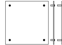
kit 105 V (kit B 30 / kit B 50) w 500 x h 500 x d 8mm w 19,69 x h 19,69 x d 0,31"
