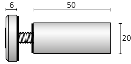
kit A 50 Ø 30 x d 6 - Ø 20 x d 50mm Ø 1,18 x d 0,24" - Ø 0,79 x d 1,97"
