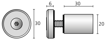
kit A 30 Ø 30 x d 6 - Ø 20 x d 30mm Ø 1,18 x d 0,24" - Ø 0,79 x d 1,18"
