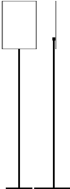
ski 905 w 215 x h 1230 x d 270 w 8,46 x h 48,42 x d 10,63"
